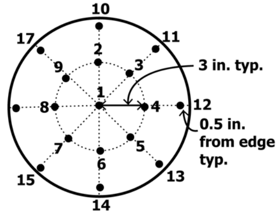
FIG. 1 Thermocouple Placement
