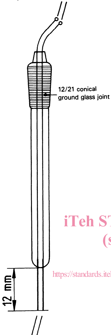
Figure 3 — Platinum electrodes
