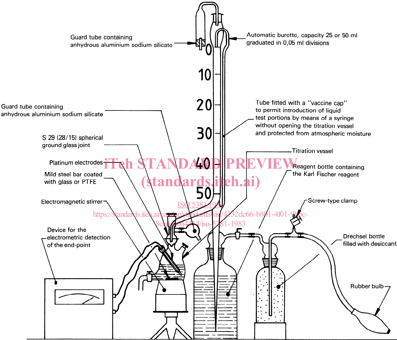
Figure 2 – General arrangement
