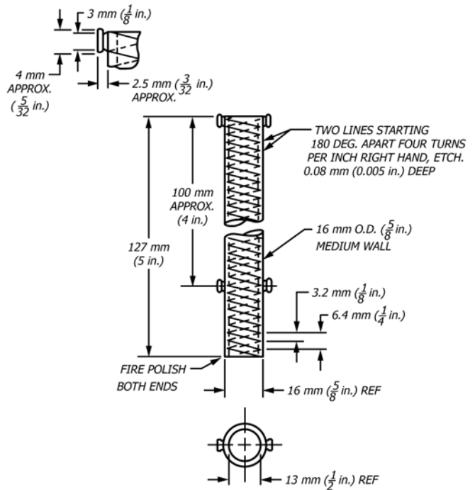
FIG. 2 Glass Tube
