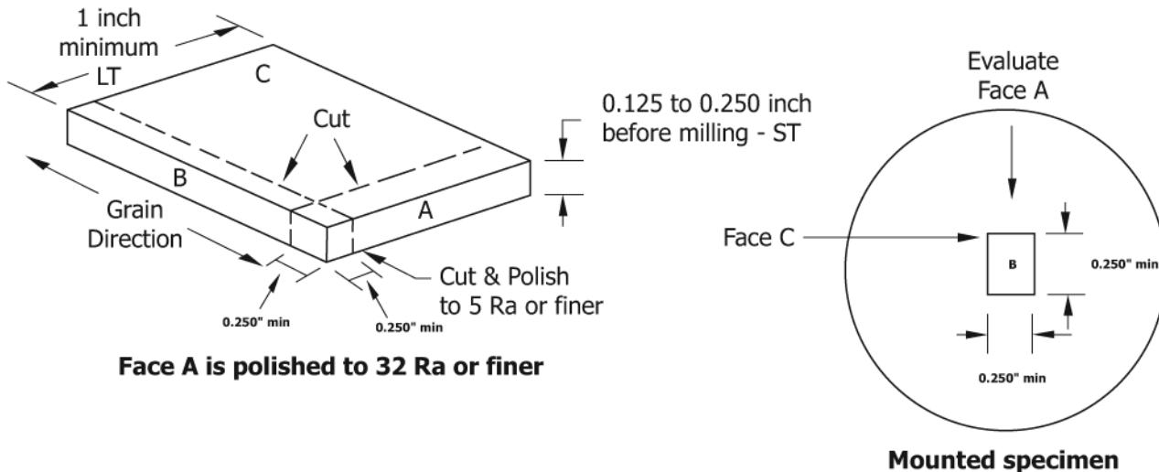
FIG. 1 Test Specimen
