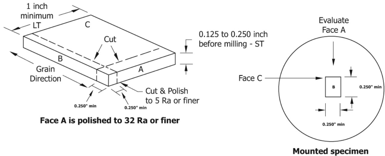
FIG. 1 Test Specimen
