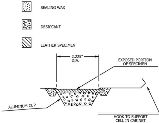
FIG. 1 Permeability Apparatus
