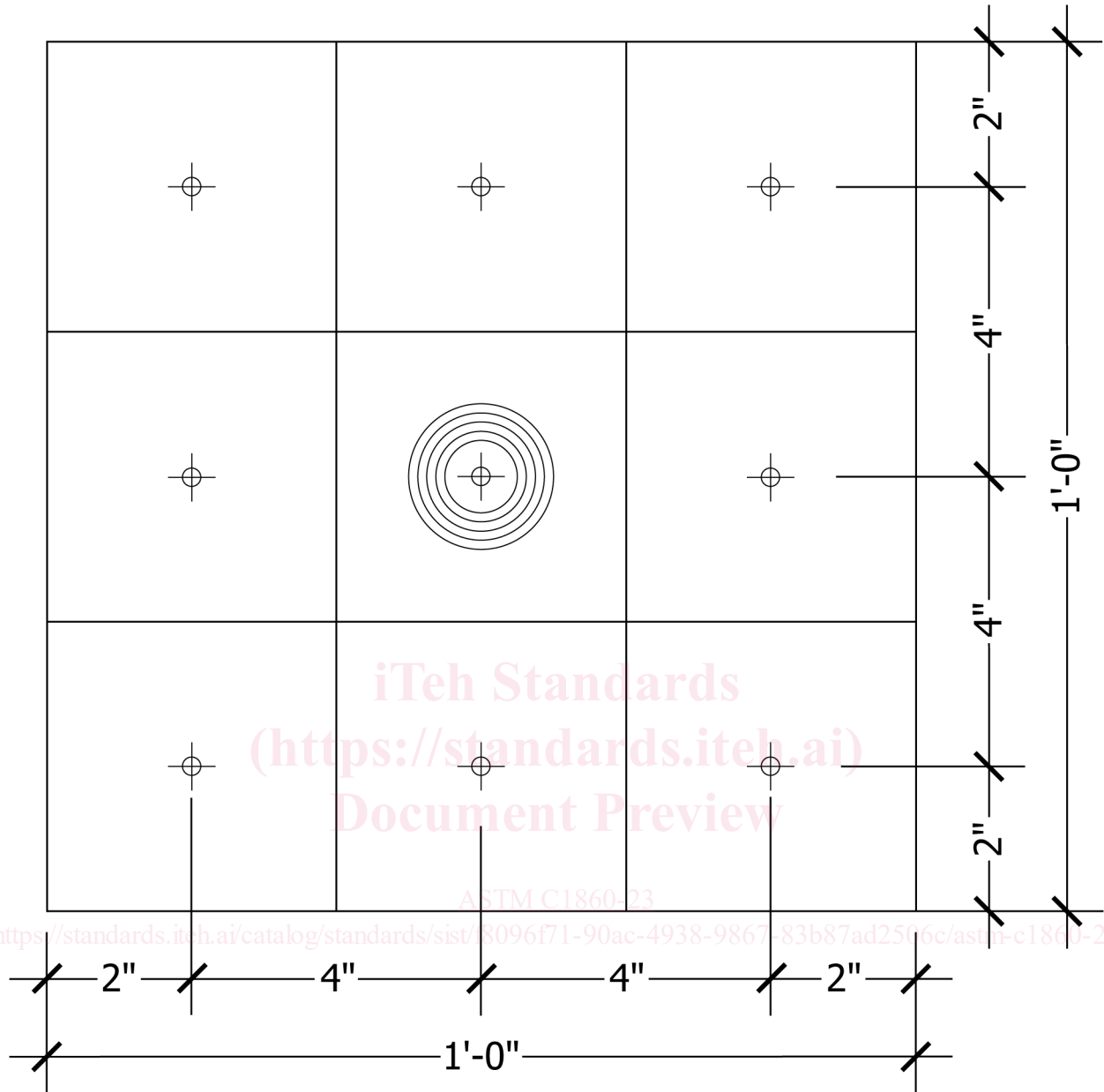
(8) #14 1/4" DIAM. x 7/8" WOOD LAG SCREWS
