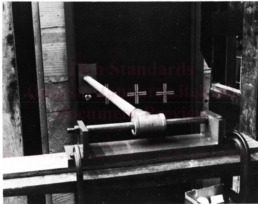
FIG. 5 Vertical Impactor
