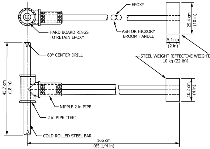
FIG. 6 Vertical Impactor Pendulum System
