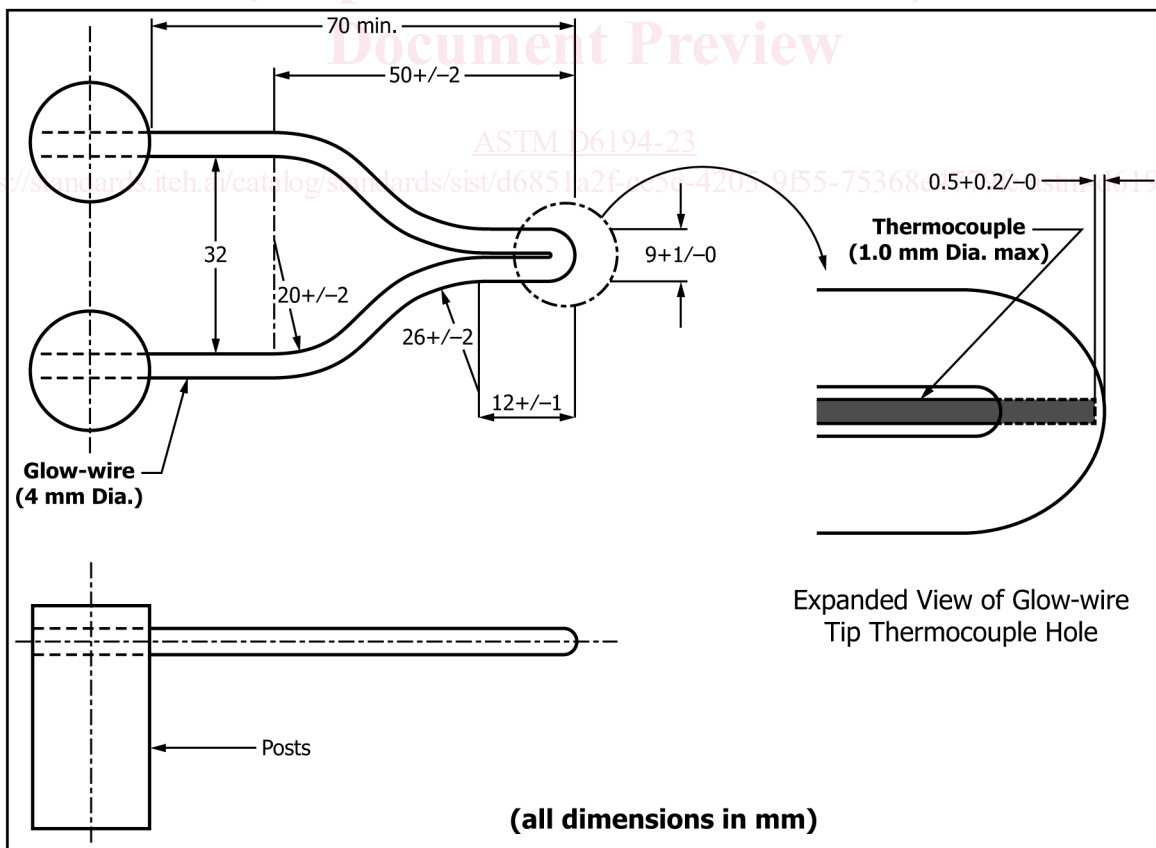
NOTE 1—All dimensions in millimetres. FIG. 1 Glow-Wire and Positioning of Thermocouple
