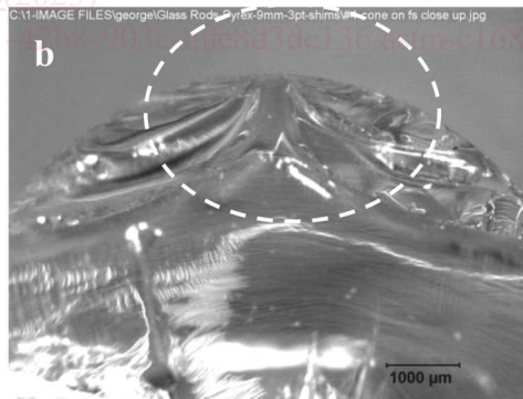
NOTE 1—The maximum tensile stress was on the bottom dead center in each case. In (a), the fracture origin is slightly to the left (arrow). A harmless contact crack (circled) on the compression half of the rod is exposed by the primary fracture. (b) shows close-up of the latter from another specimen.
