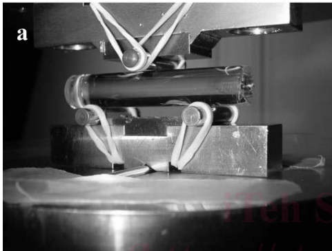
NOTE 1—(a) shows three-point loading of a 9-mm diameter short glass specimen with 4.5-mm steel rollers and a 30-mm span. Note that the bottom of the fixture does not need to articulate in three-point bending. (b) shows a Hertzian contact crack in the surface of the glass rod.
