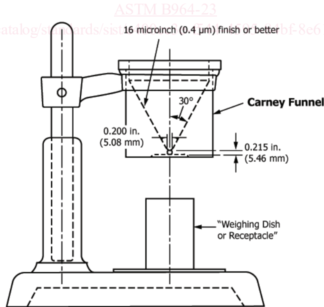
FIG. 1 Carney Funnel and Stand
