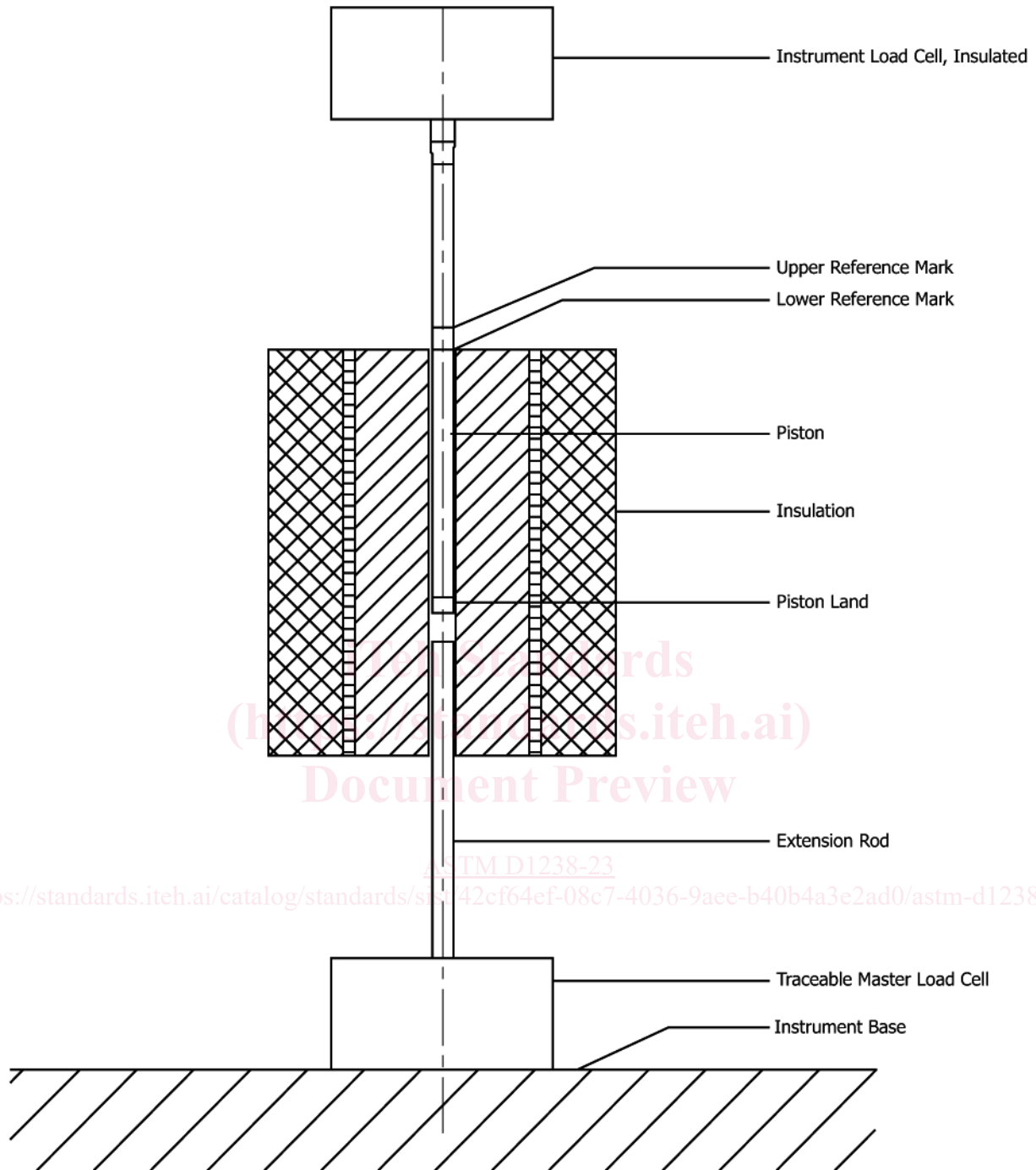
FIG. 3 Calibration Set-Up
