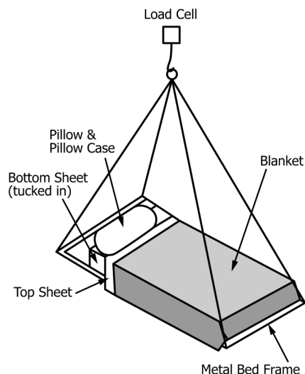
FIG. 7 Bed Assembly With Suspending Strain Gauge Load Cell
