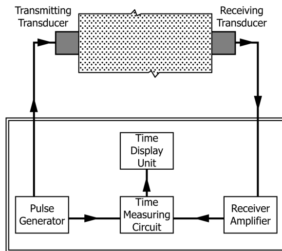
FIG. 1 Schematic of Ultrasonic Pulse Velocity Apparatus
