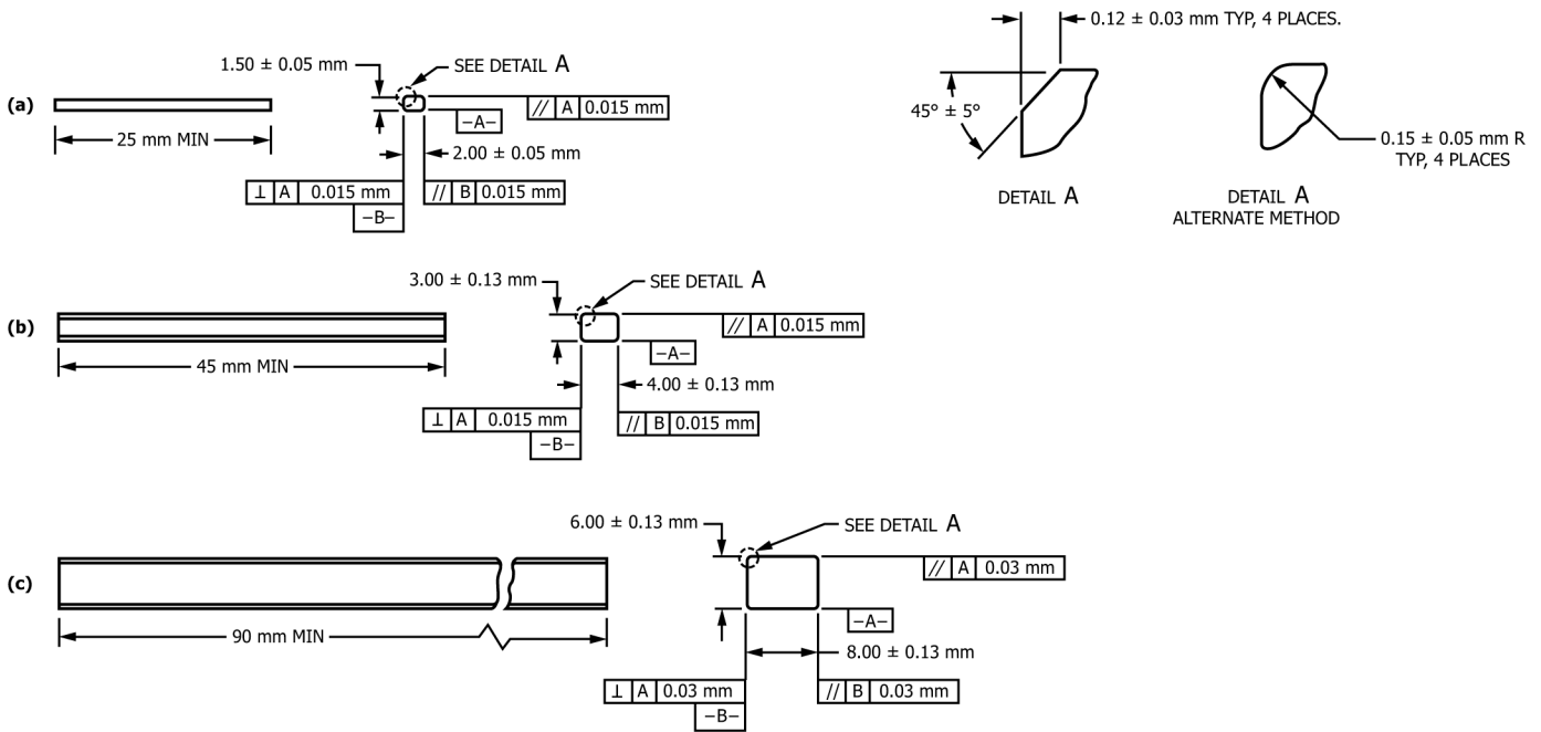
FIG. 4 Standard Test Specimens
