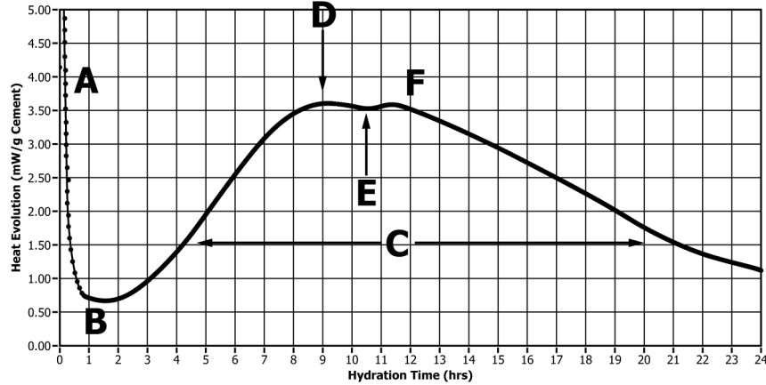
FIG. 1 Example of Thermal Power Curve for Isothermal Hydration of Portland Cement
