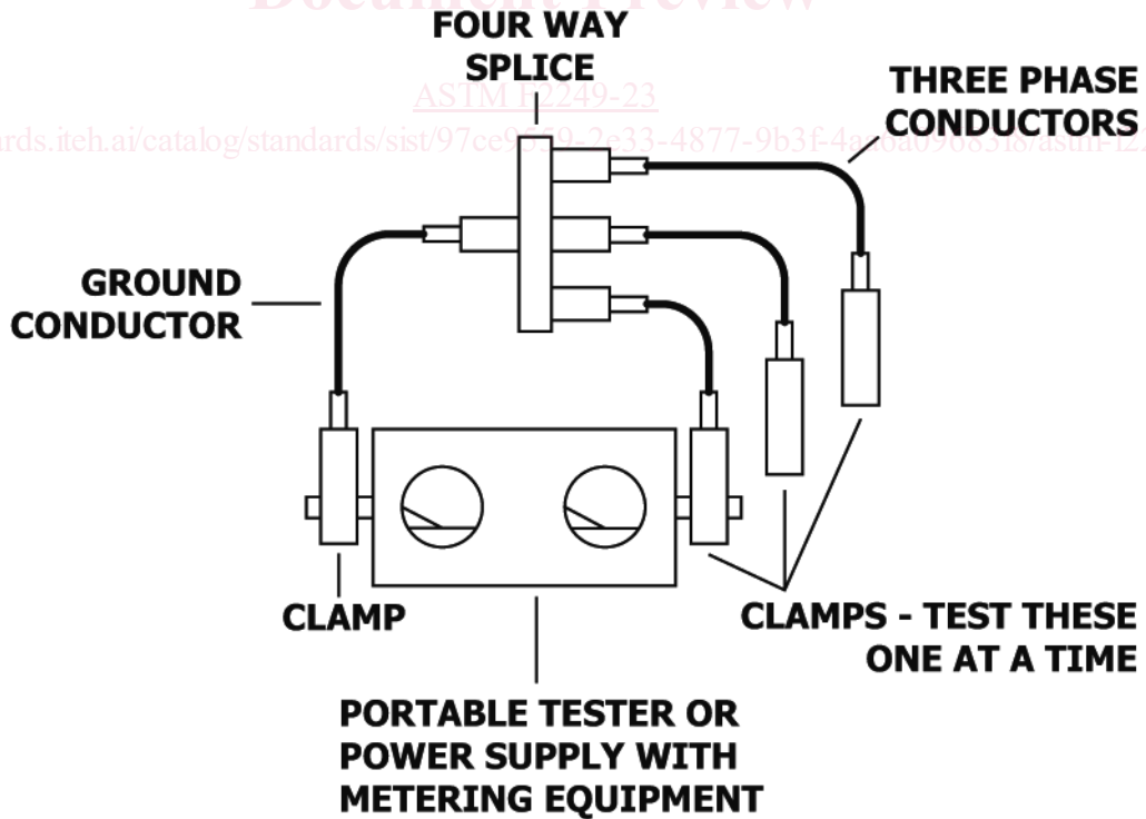
FIG. 2 Typical Configurations
