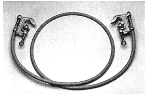
FIG. 8 Style II—Assembled Flexible By-Pass Jumper Designed and Manufactured to be Installed with Live Line Tools
