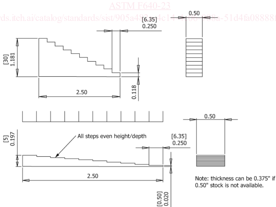
FIG. 1 Example Dimensions of Aluminum Step Wedges
