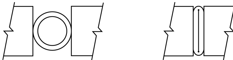
1 – PLACE THE INSERT IN A VISE OR OTHER SUITABLE DEVICE. 2 – CLOSE THE VICE JAWS UNTIL THE INSIDE WALLS TOUCH.
