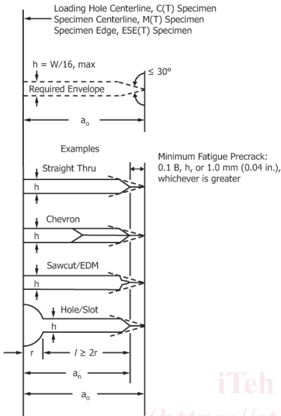
FIG. 1 Notch Details and Minimum Fatigue Precracking Requirements
