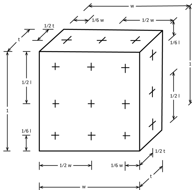
FIG. 4 Measurement Locations for Determining Test Specimen Dimensions
