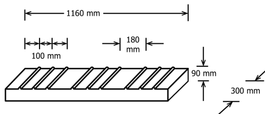
(a) Typical dimensions for an immersion tank
