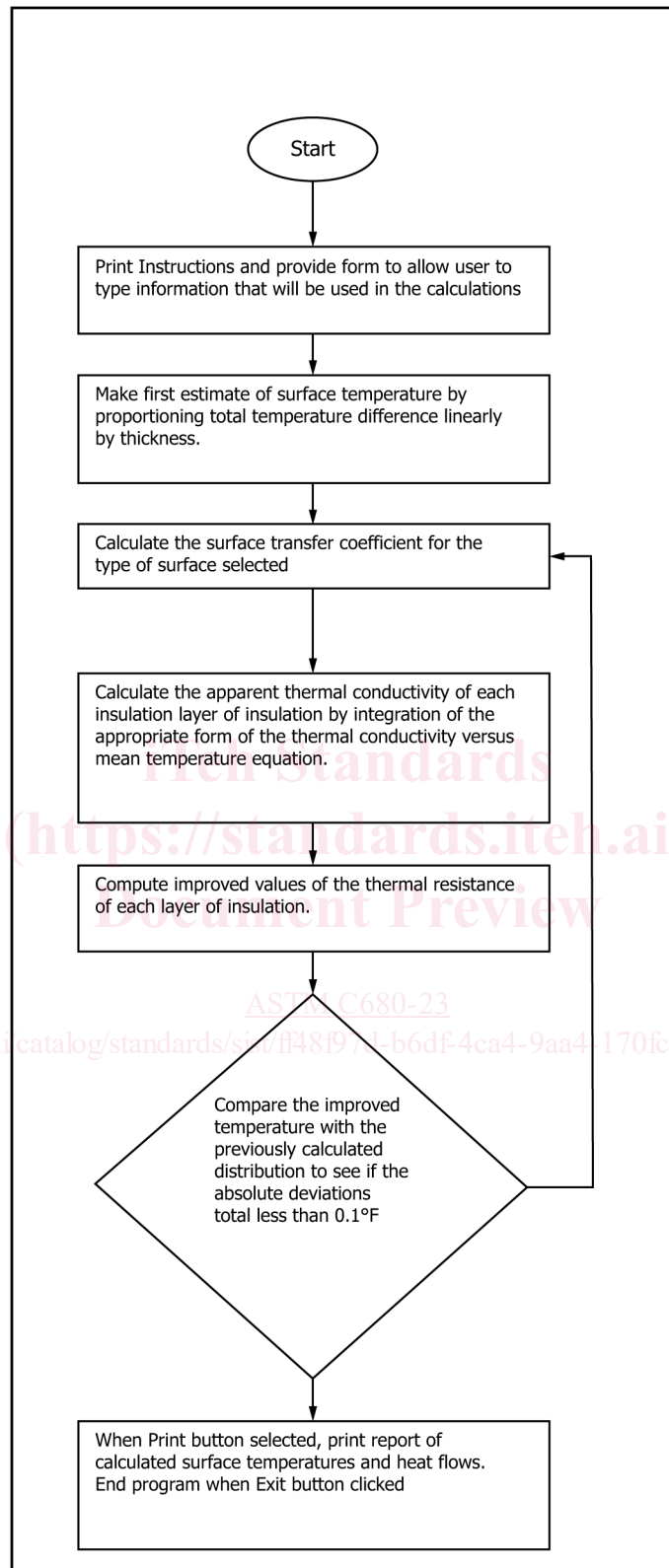
FIG. 1 Flow Chart
