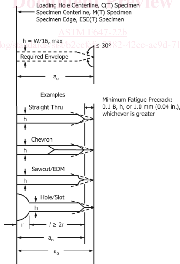
FIG. 42 Notch Details and Minimum Fatigue Precracking Requirements
