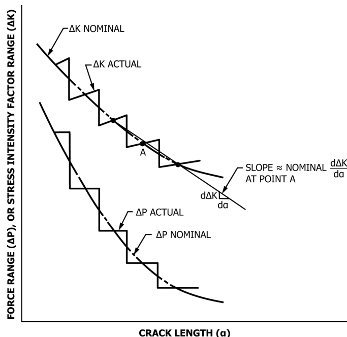
FIG. 23 Typical K Decreasing Test by Stepped Force Shedding
