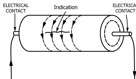
FIG. 3 Circular Magnetization, Current Directly Through Forging
