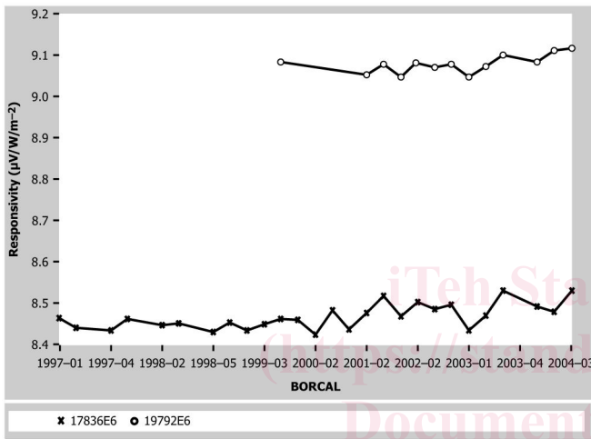
FIG. 1 Typical Within Laboratory Precision for Lab A (left) and Lab B (right) for Pyrheliometer Calibrations
