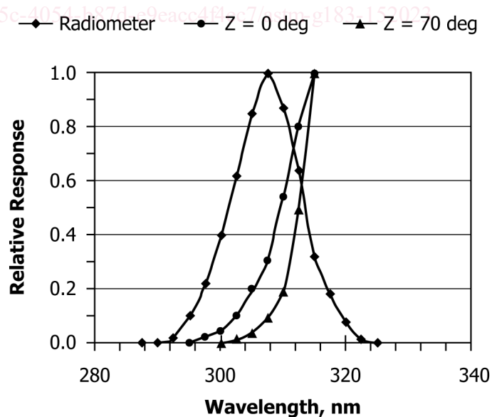
FIG. X1.1 UV-B Radiometer Response and UV-B Solar Spectral Distribution at Two Zenith Angles
