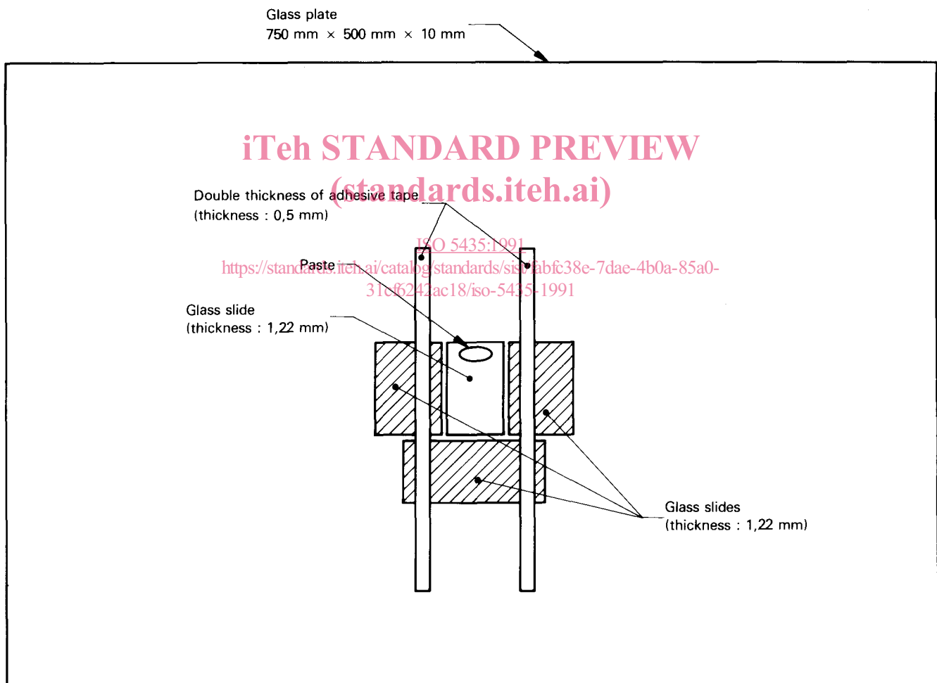
Figure 1 — Slide preparation apparatus for Meeco Colormaster
