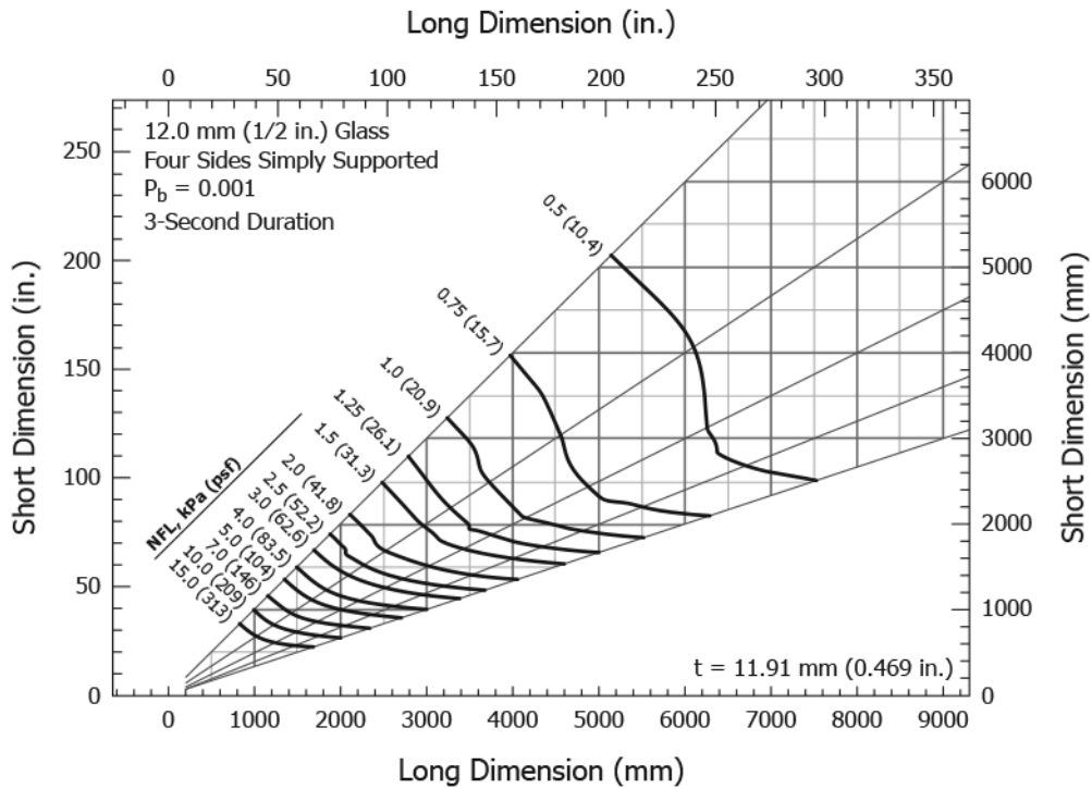
FIG. A1.4 Load Resistance Chart for 12 mm (1/2 in.) Annealed Monolithic Glass Continuously Supported Along Four Sides ( P_b = 0.001 )
