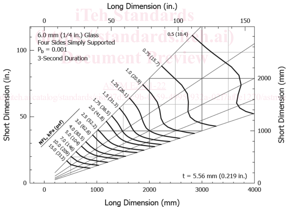
FIG. A1.1 Load Resistance Chart for 6 mm (1/4 in.) Annealed Monolithic Glass Continuously Supported Along Four Sides ( P_b = 0.001 )
