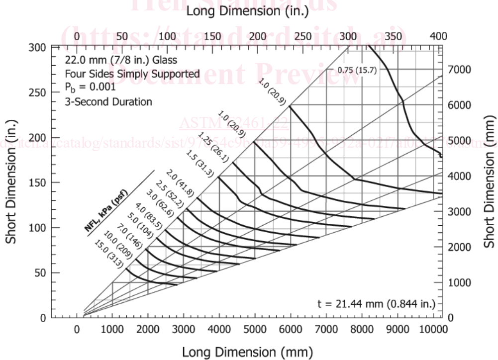
FIG. A1.7 Load Resistance Chart for 22 mm (7/8 in.) Annealed Monolithic Glass Continuously Supported Along Four Sides ( P_b = 0.001 )
