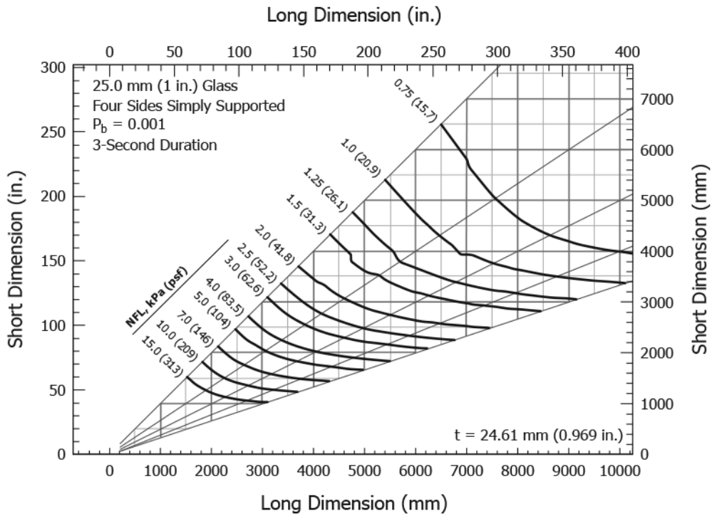
FIG. A1.8 Load Resistance Chart for 25 mm (1 in.) Annealed Monolithic Glass Continuously Supported Along Four Sides ( P_b = 0.001 )
