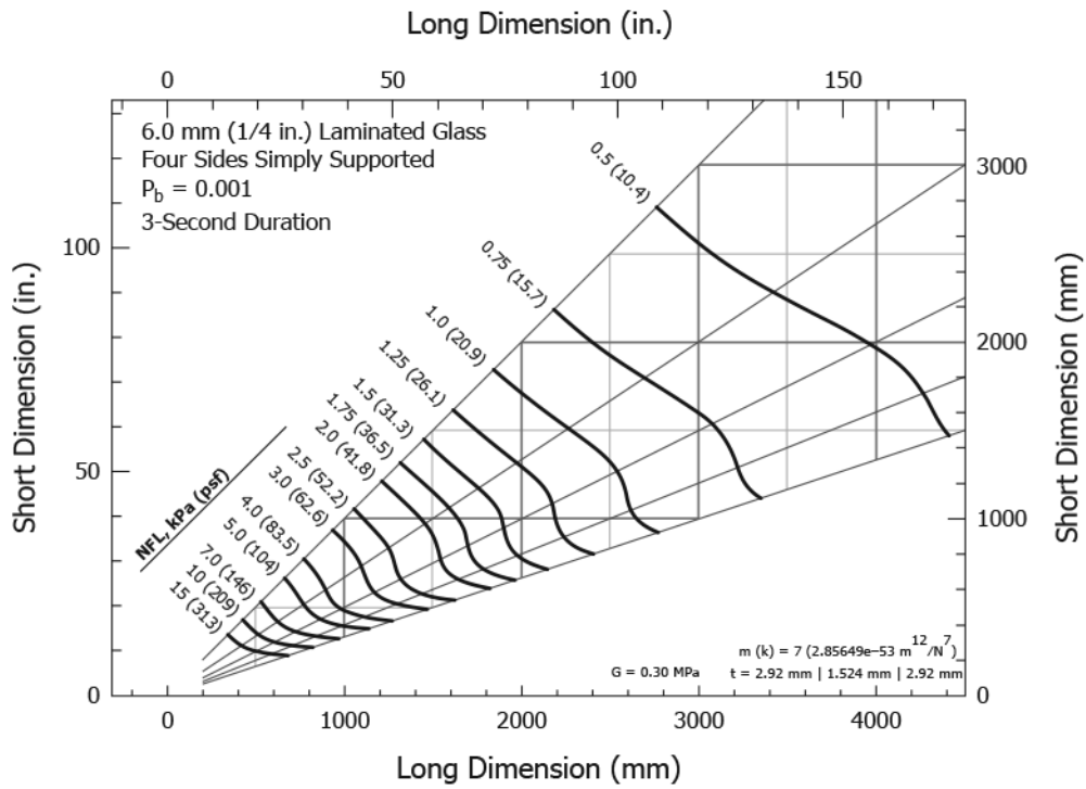
FIG. A1.17 b Load Resistance Chart for 6 mm (1/4 in.) Annealed Laminated Glass Continuously Supported Along Four Sides ( P_b = 0.001 ) (continued)
