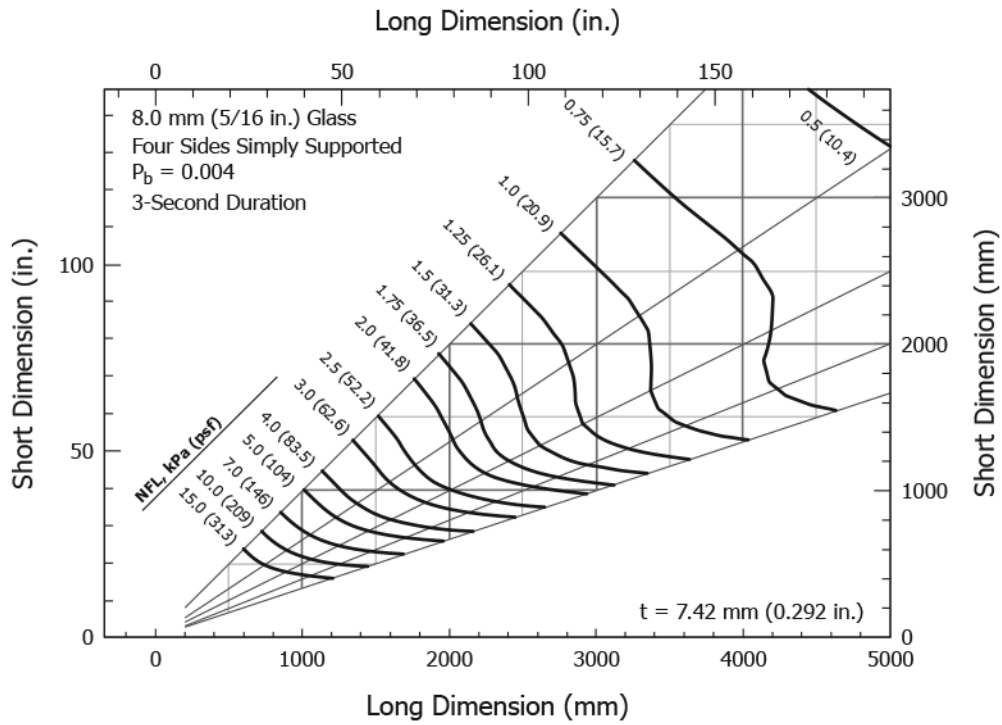
FIG. A1.10 Load Resistance Chart for 8 mm (5/16 in.) Annealed Monolithic Glass Continuously Supported Along Four Sides ( P_b = 0.004 )
