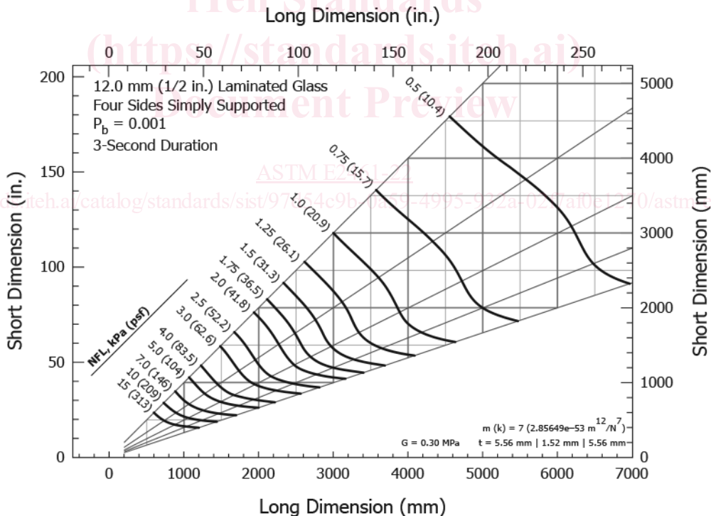
FIG. A1.20 Load Resistance Chart for 12 mm (1/2 in.) Annealed Laminated Glass Continuously Supported Along Four Sides ( P_b = 0.001 )
