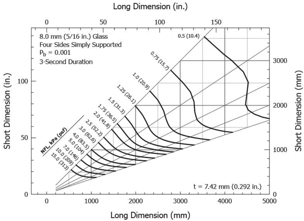
FIG. A1.2 Load Resistance Chart for 8 mm (5/16 in.) Annealed Monolithic Glass Continuously Supported Along Four Sides ( P_b = 0.001 )
