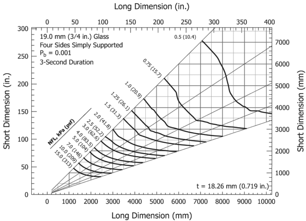
FIG. A1.6 Load Resistance Chart for 19 mm (3/4 in.) Annealed Monolithic Glass Continuously Supported Along Four Sides ( P_b = 0.001 )
