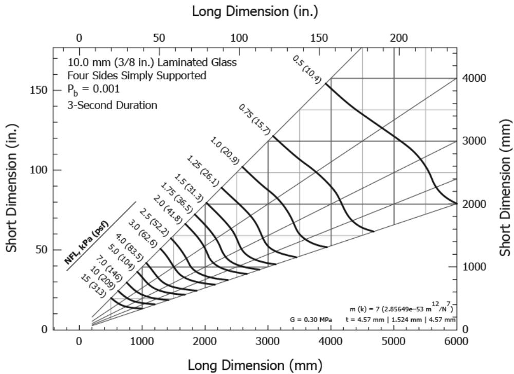
FIG. A1.19 Load Resistance Chart for 10 mm (3/8 in.) Annealed Laminated Glass Continuously Supported Along Four Sides ( P_b = 0.001 )
