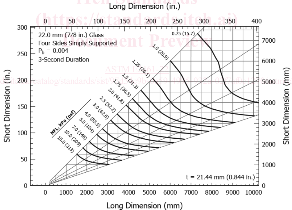
FIG. A1.15 Load Resistance Chart for 22 mm (7/8 in.) Annealed Monolithic Glass Continuously Supported Along Four Sides ( P_b = 0.004 )
