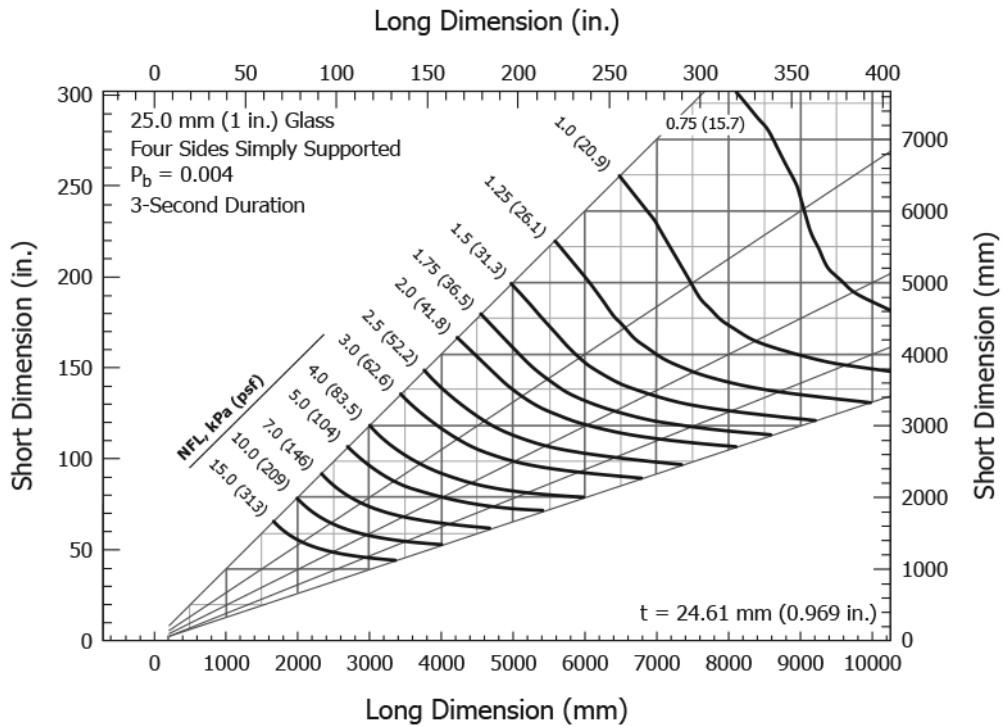
FIG. A1.16 Load Resistance Chart for 25 mm (1 in.) Annealed Monolithic Glass Continuously Supported Along Four Sides ( P_b = 0.004 )
