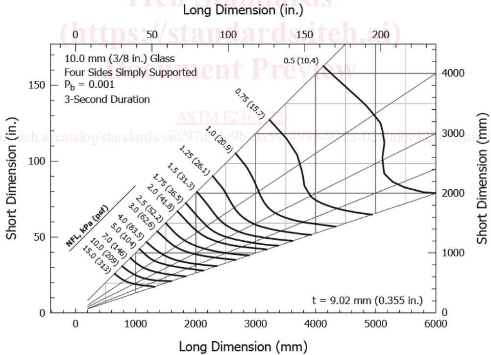
FIG. A1.3 Load Resistance Chart for 10 mm (3/8 in.) Annealed Monolithic Glass Continuously Supported Along Four Sides ( P_b = 0.001 )
