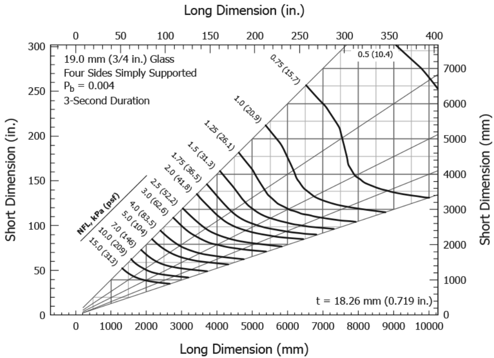
FIG. A1.14 Load Resistance Chart for 19 mm (3/4 in.) Annealed Monolithic Glass Continuously Supported Along Four Sides ( P_b = 0.004 )
