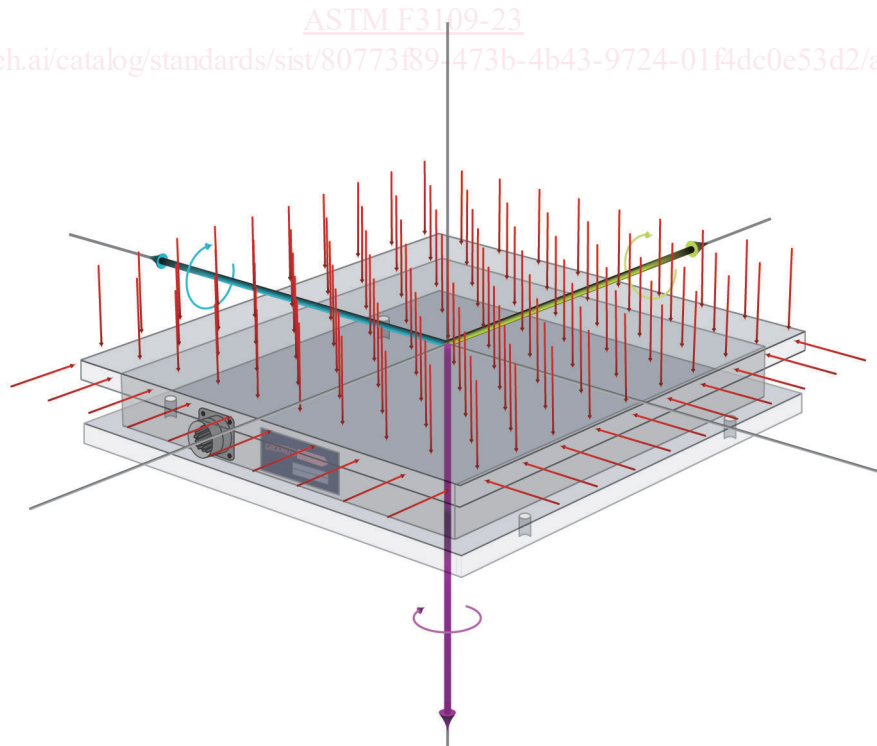
FIG. 2 Illustration of Spatial Grid Pattern Used to Apply Forces for Force Platform Verification
