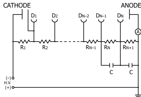
FIG. 4 Voltage-Divider Bridge
