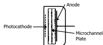
FIG. 2 Electrostatic Dynode Structures
