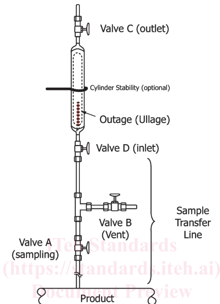
FIG. 2 Typical Sample Container and Alternate Purging Connections (Inverted)
