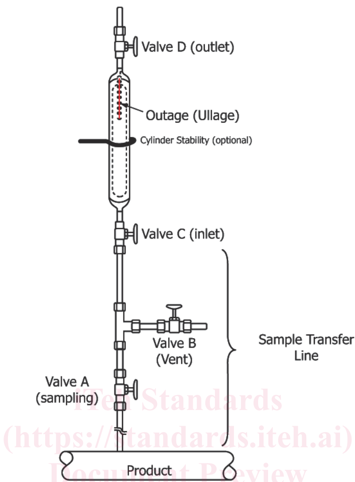
FIG. 1 Typical Sample Container and Sampling Connections (Upright)
