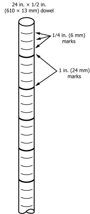
FIG. 3 Dowel Markings
