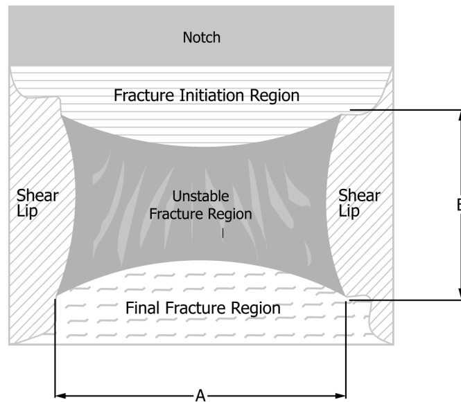
NOTE 1—Measure average dimensions A and B to the nearest 0.5 mm. Determine the shear fracture appearance using Table A4.1 or Table A4.2. FIG. 9 Schematic of the Fracture Surface of a Charpy V-Notch Impact Test Specimen Showing the Various Region of Fracture
