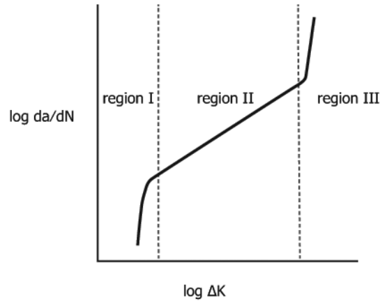
FIG. 1 Defined Regions of a Typical Fatigue Crack Growth Rate Curve
