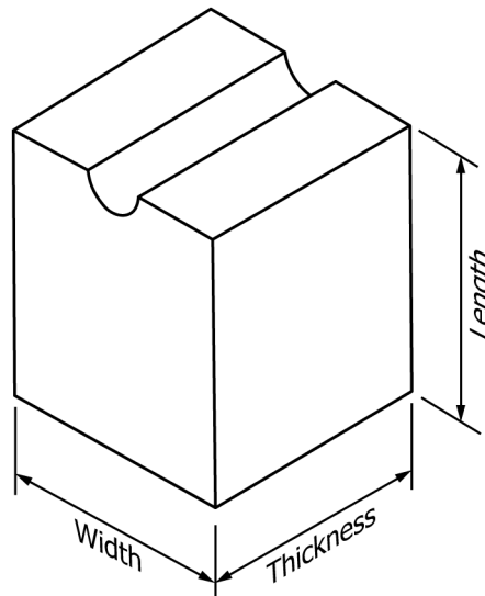
FIG. 1 Specimen Configuration – Half-Hole
