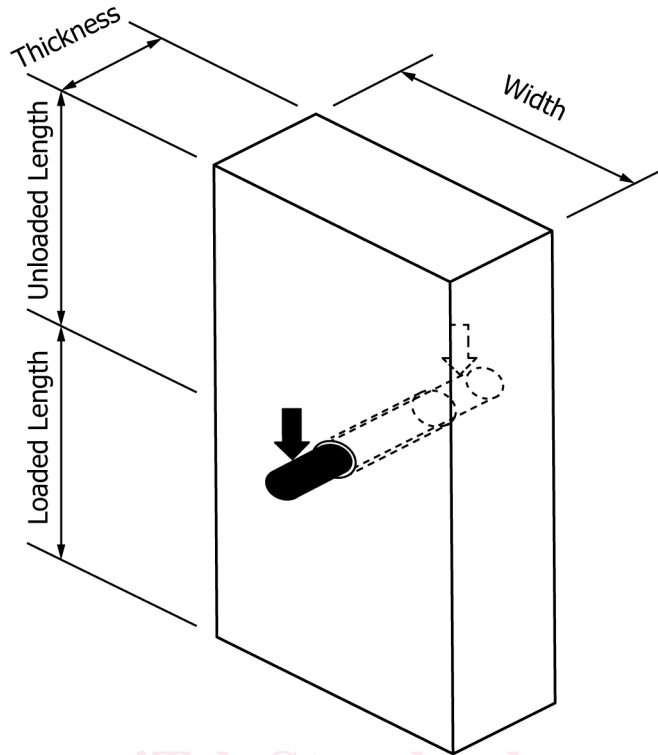
FIG. 32 Specimen Configuration—Full Hole Configuration — Full-Hole
