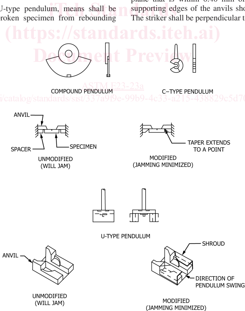
FIG. A1.1 Typical Pendulums and Anvils for Charpy Machines, Shown with Modifications to Minimize Jamming
