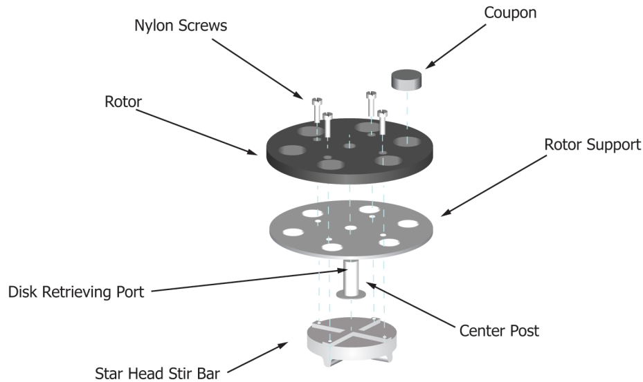
FIG. 2 Rotor Assembly
