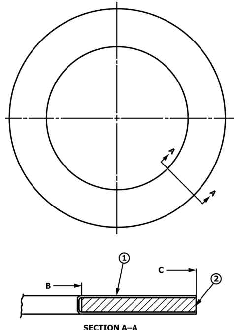
FIG. 5 Folded Design (Flat Ring)
