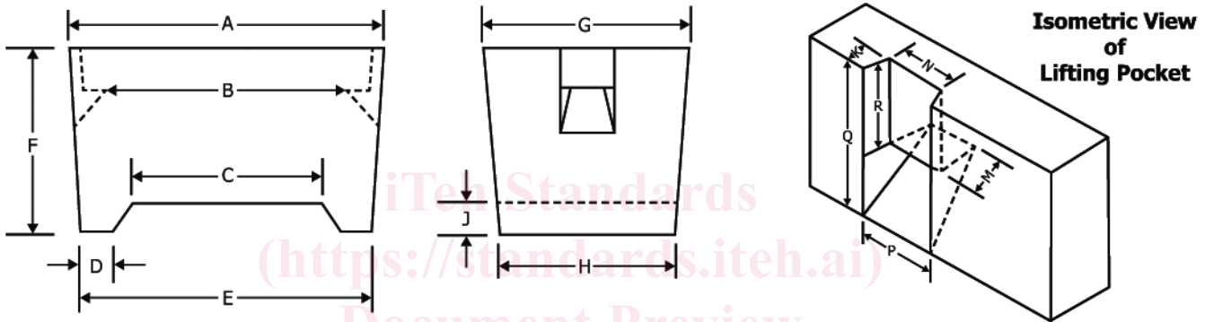
FIG. 2 Type 1 Block Ingot
