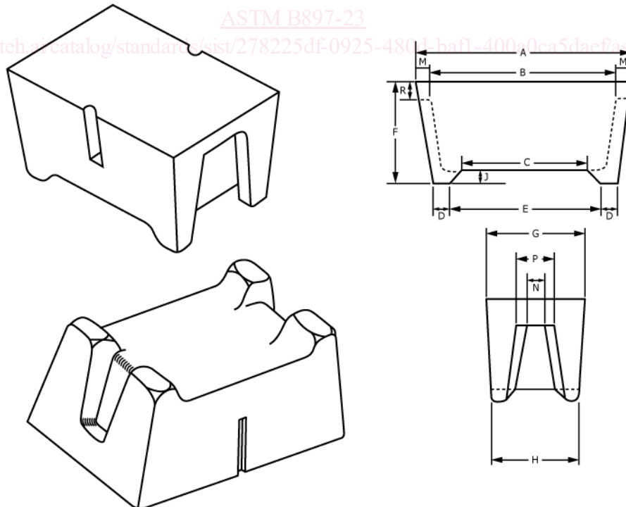
FIG. 3 Type 2 Block Ingot
