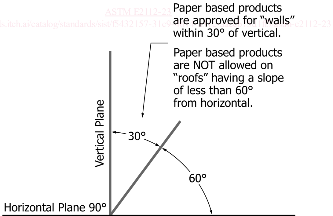
FIG. 2 Flashing on Sloped Surfaces
