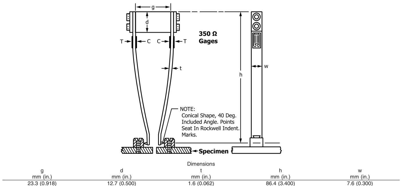
FIG. 3 Enlarged Clip Gage for Compliance Measurements on Large Specimens
