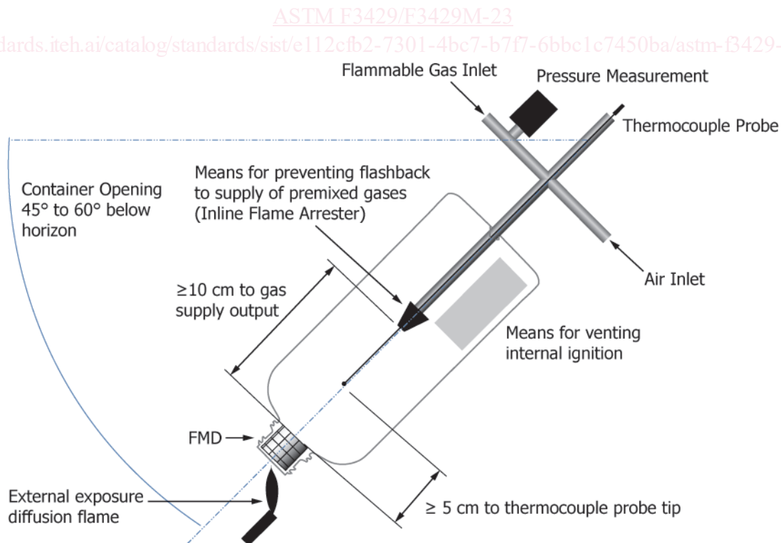
FIG. 1 Example Setup of Container for Endurance Test Method, Using a Thermocouple Probe and Pressure Measurement
