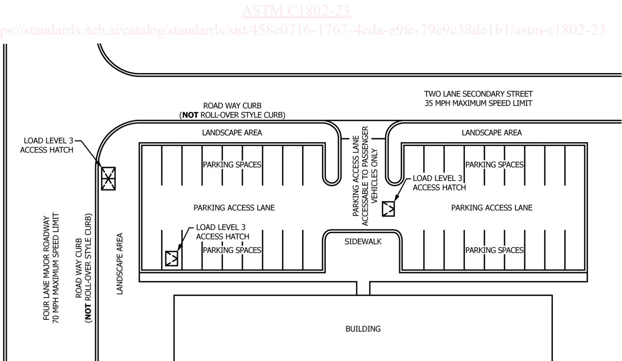
FIG. 3 Plan Showing Appropriate Locations for Load Level 3 Access Hatches—Light Vehicular Traffic
