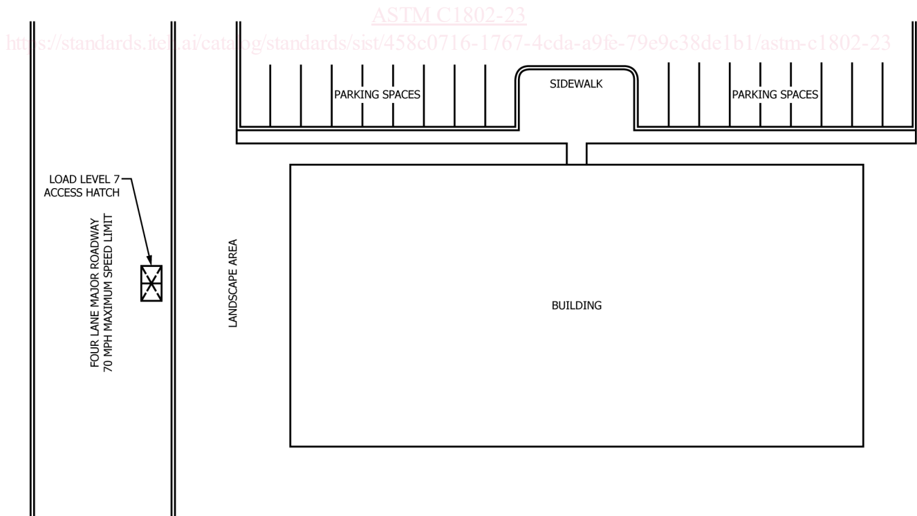
FIG. 7 Plan Showing Appropriate Locations for Load Level 7 Access Hatches—Full Traffic
