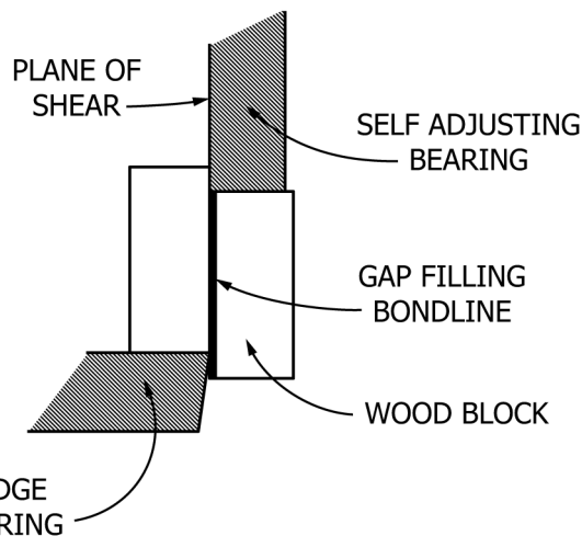
FIG. 3 Side View of Test Specimen Showing Method of Notching Specimen to Ensure Proper Alignment of Shearing Tool and Plane of Shear
