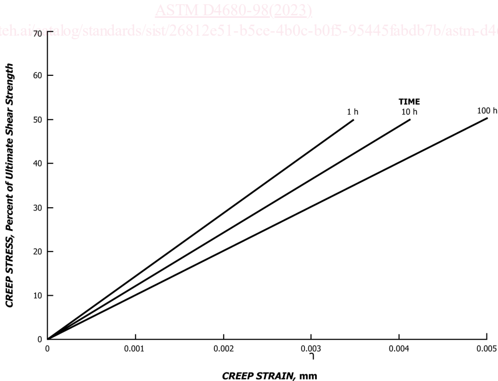
FIG. 3 Stress-Strain Curves at Various Times
