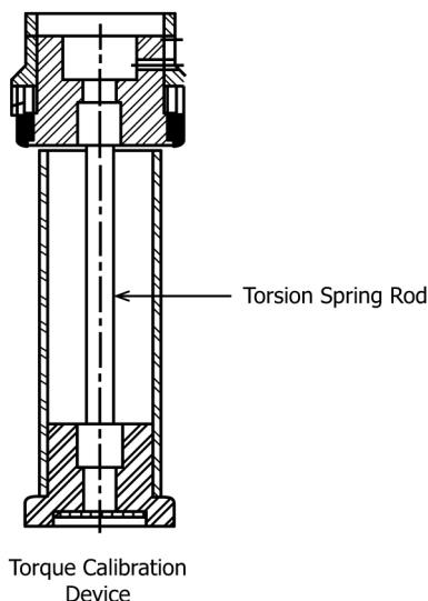
FIG. 4 Typical Torque Standard torque calibration device used to calibrate the torque measurement system in an encapsulated specimen parallel plate rheometer.
