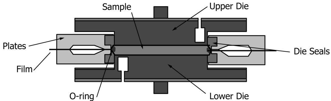
FIG. 1 Encapsulated specimen parallel plate rheometer plate system designed to keep a constant fiberreinforcement to resin ratio during a test.
