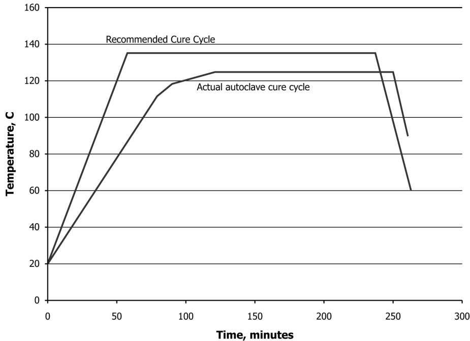
FIG. 2 Typical temperature program profile to cure components and the actual temperature at the component.
