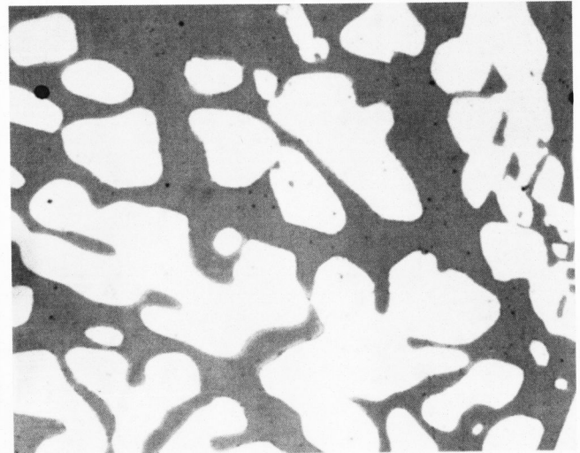
FIG. 4 (a) J92205: Possibly Affected Structure-Statically Cast (400× Magnification)
