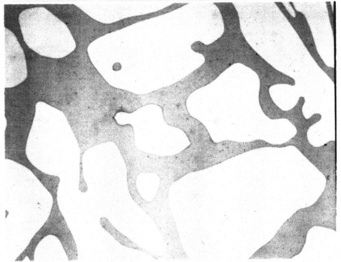
FIG. 2 (a) J92205: Unaffected Structure-Staticly Cast (400x Magnification)
