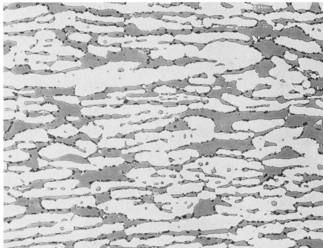
FIG. 5 Affected Structure in 8a S31803: (a) Longitudinal Section and (b) Transverse Section (500x Magnification Before Reproduction)
