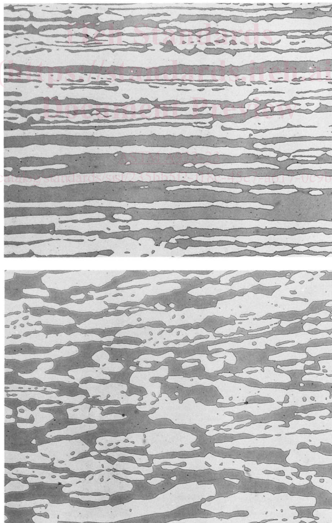
FIG. 1 Unaffected Structure in S31803: (a) Longitudinal Section and (b) Transverse Section (500x Magnification Before Reproduction)
