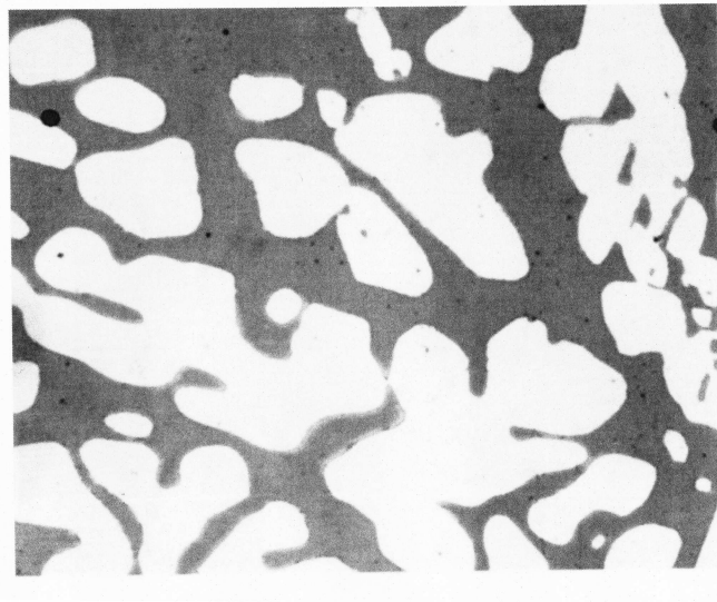
FIG. 4 (a) J92205: Possibly Affected Structure-Statically Cast (400x Magnification)
