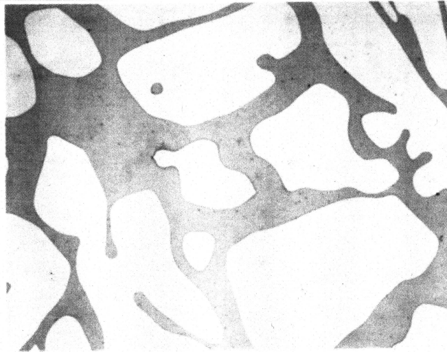
FIG. 2 (a) J92205: Unaffected Structure-Statically Cast (400× Magnification)
